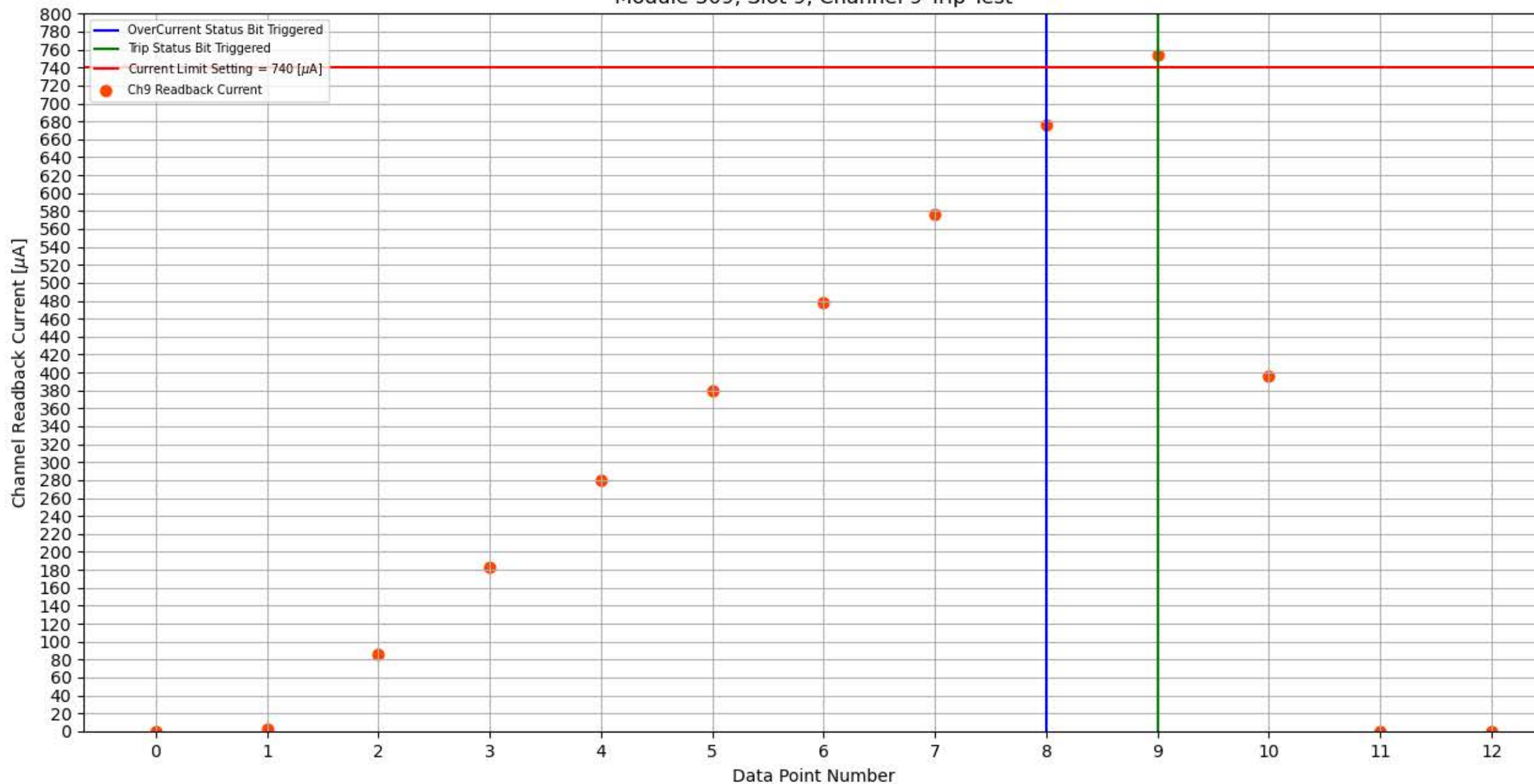
Module 309, Slot 9, Channel 9 Trip Test
