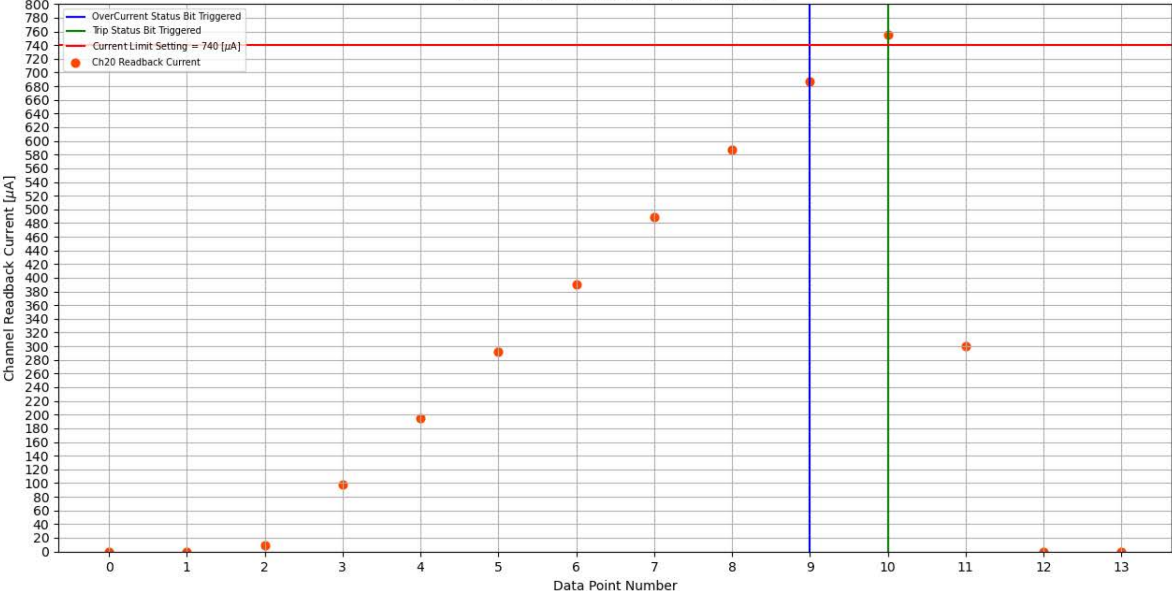
Module 309, Slot 9, Channel 20 Trip Test
