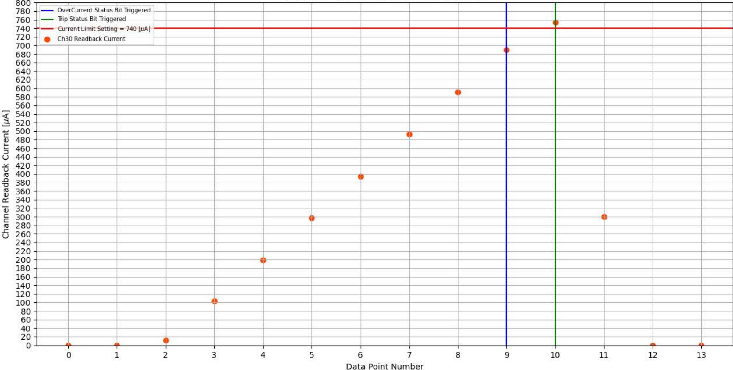
Module 309, Slot 9, Channel 30 Trip Test
