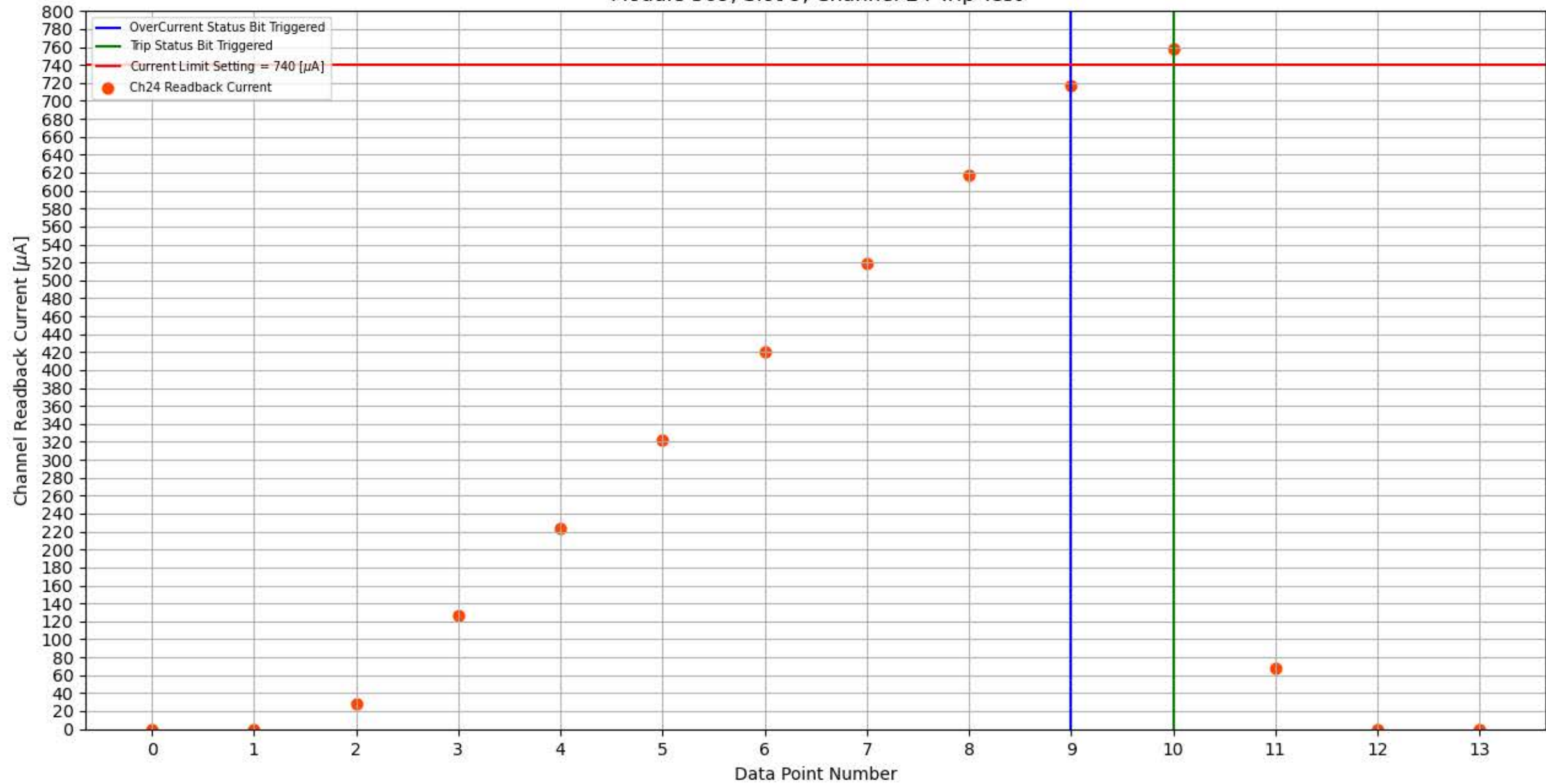
Module 309, Slot 9, Channel 24 Trip Test
