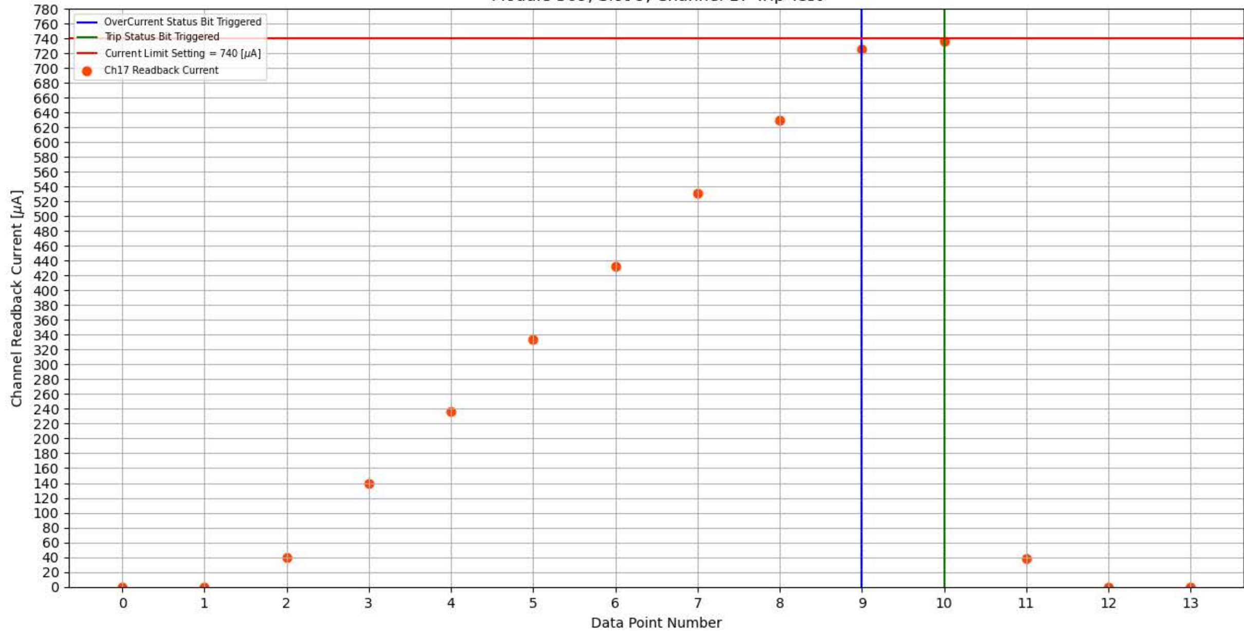
Module 309, Slot 9, Channel 17 Trip Test
