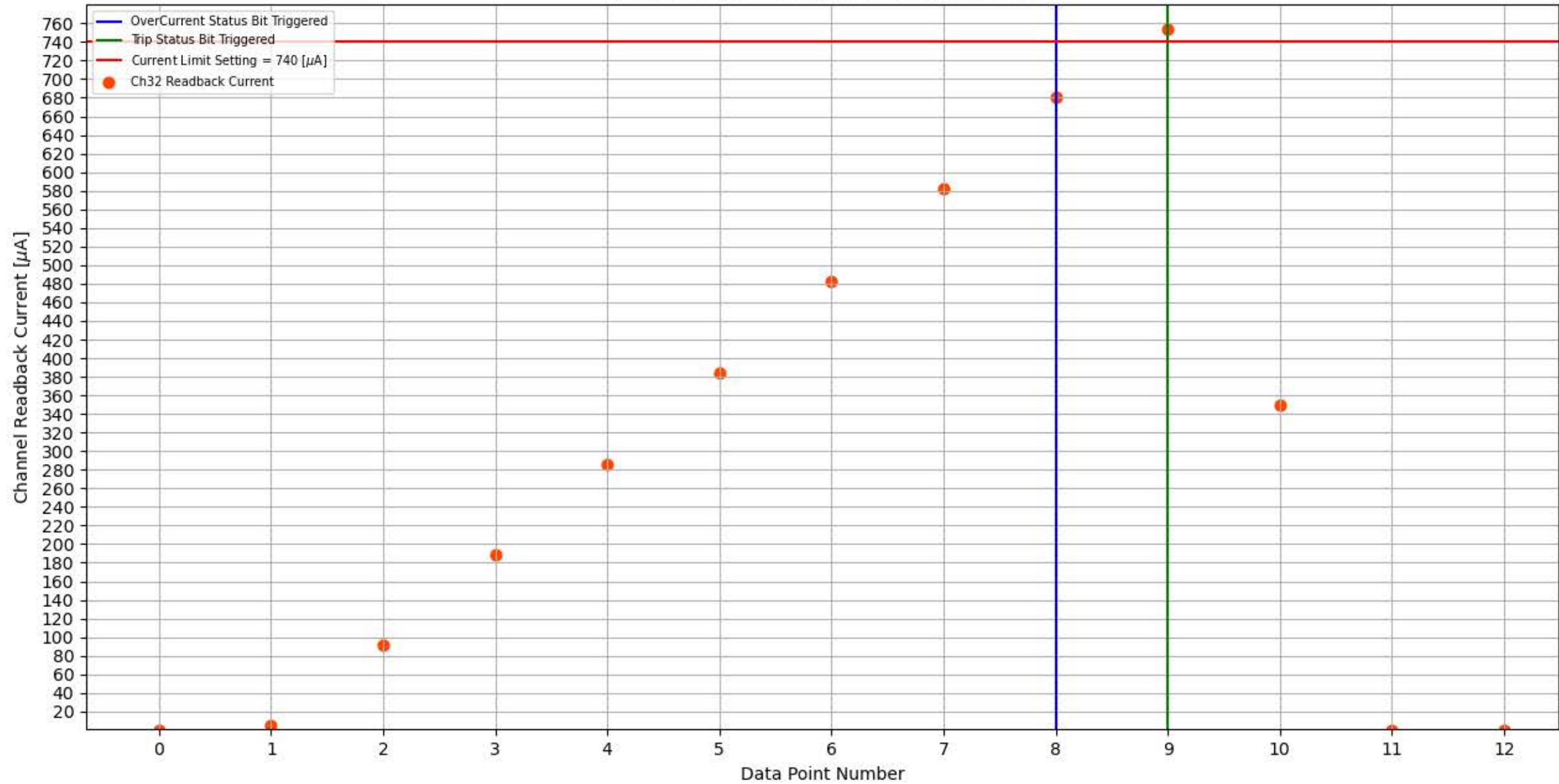
Module 309, Slot 9, Channel 32 Trip Test
