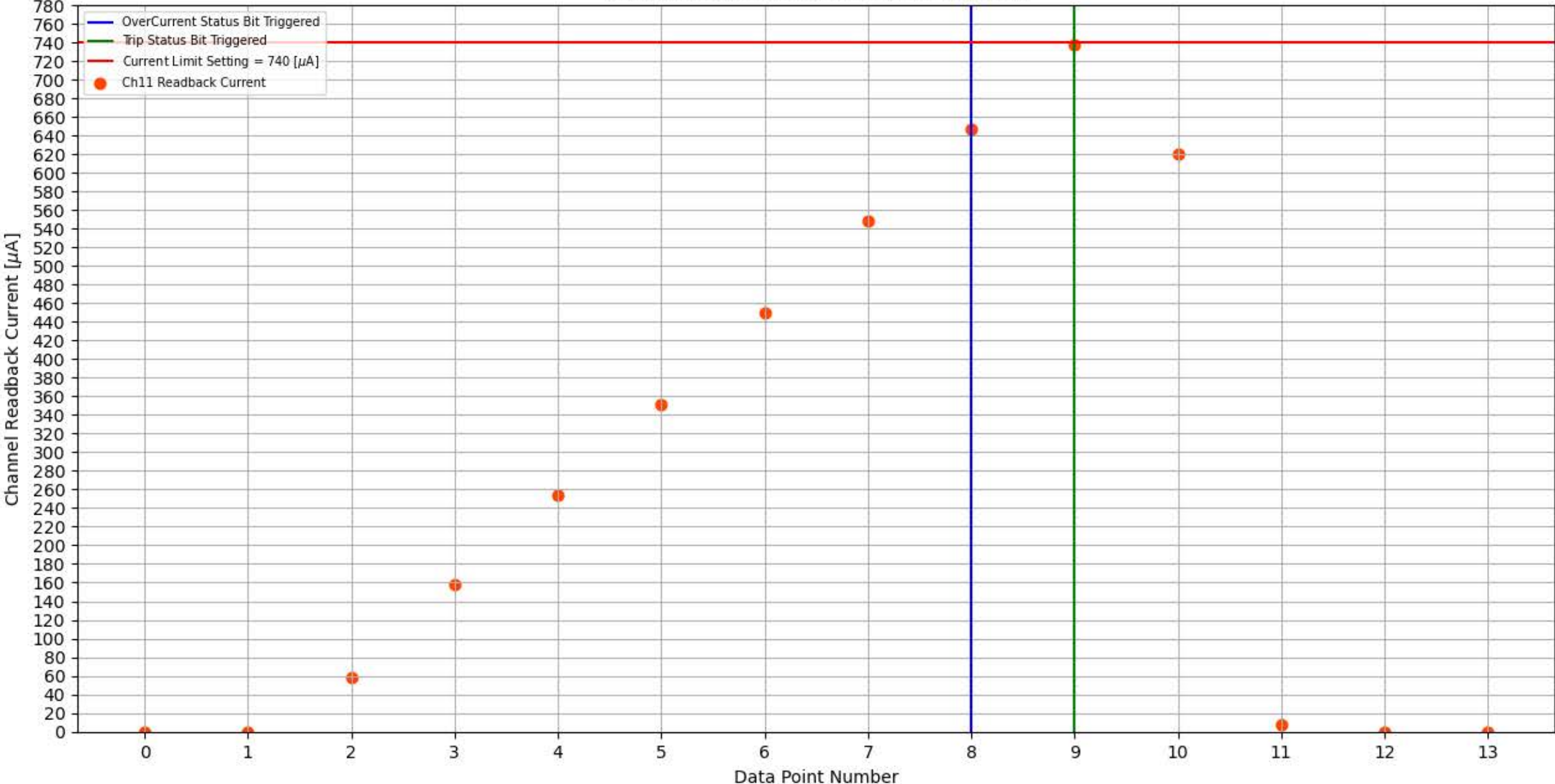
Module 309, Slot 9, Channel 11 Trip Test
