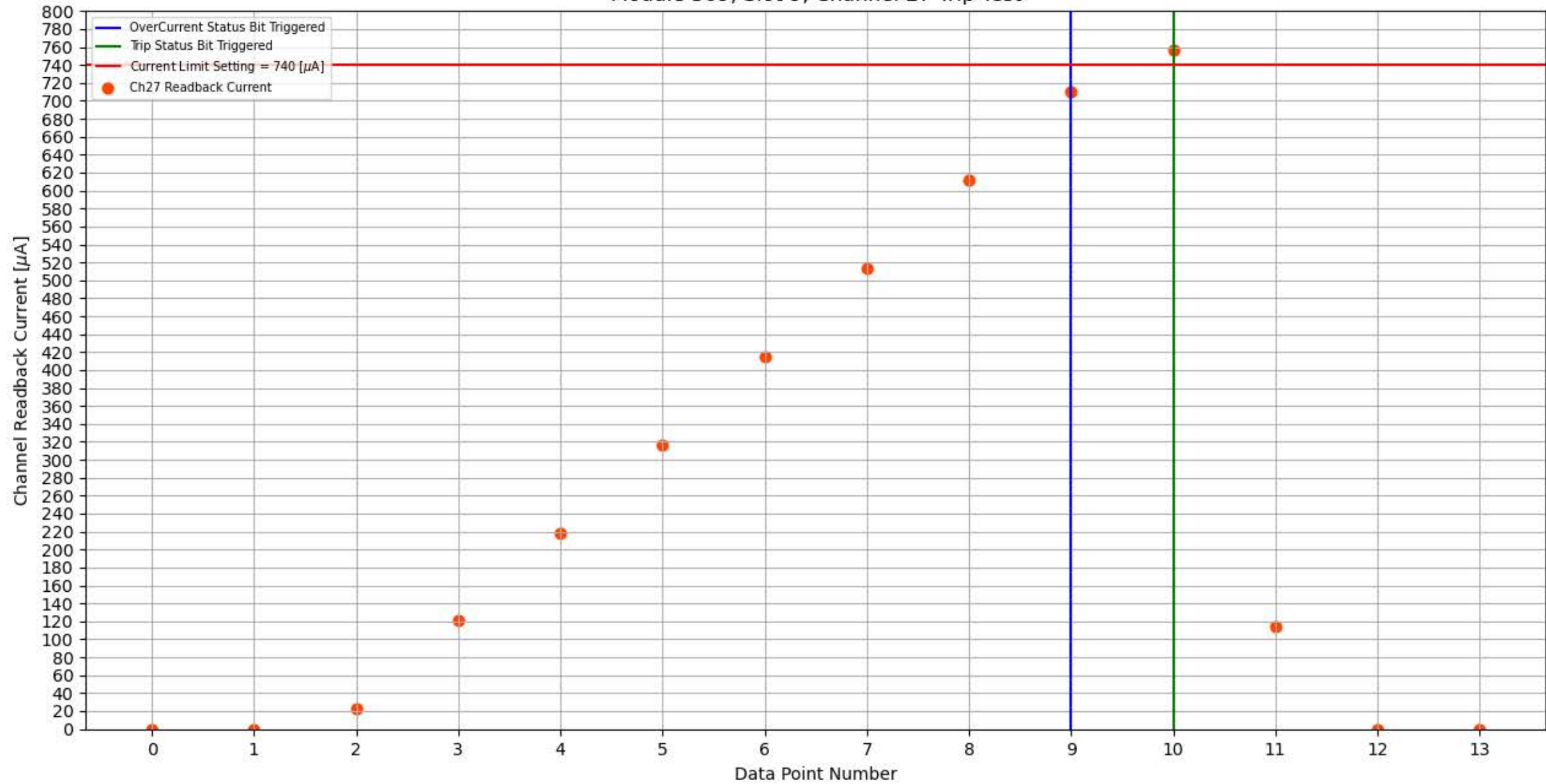
Module 309, Slot 9, Channel 27 Trip Test
