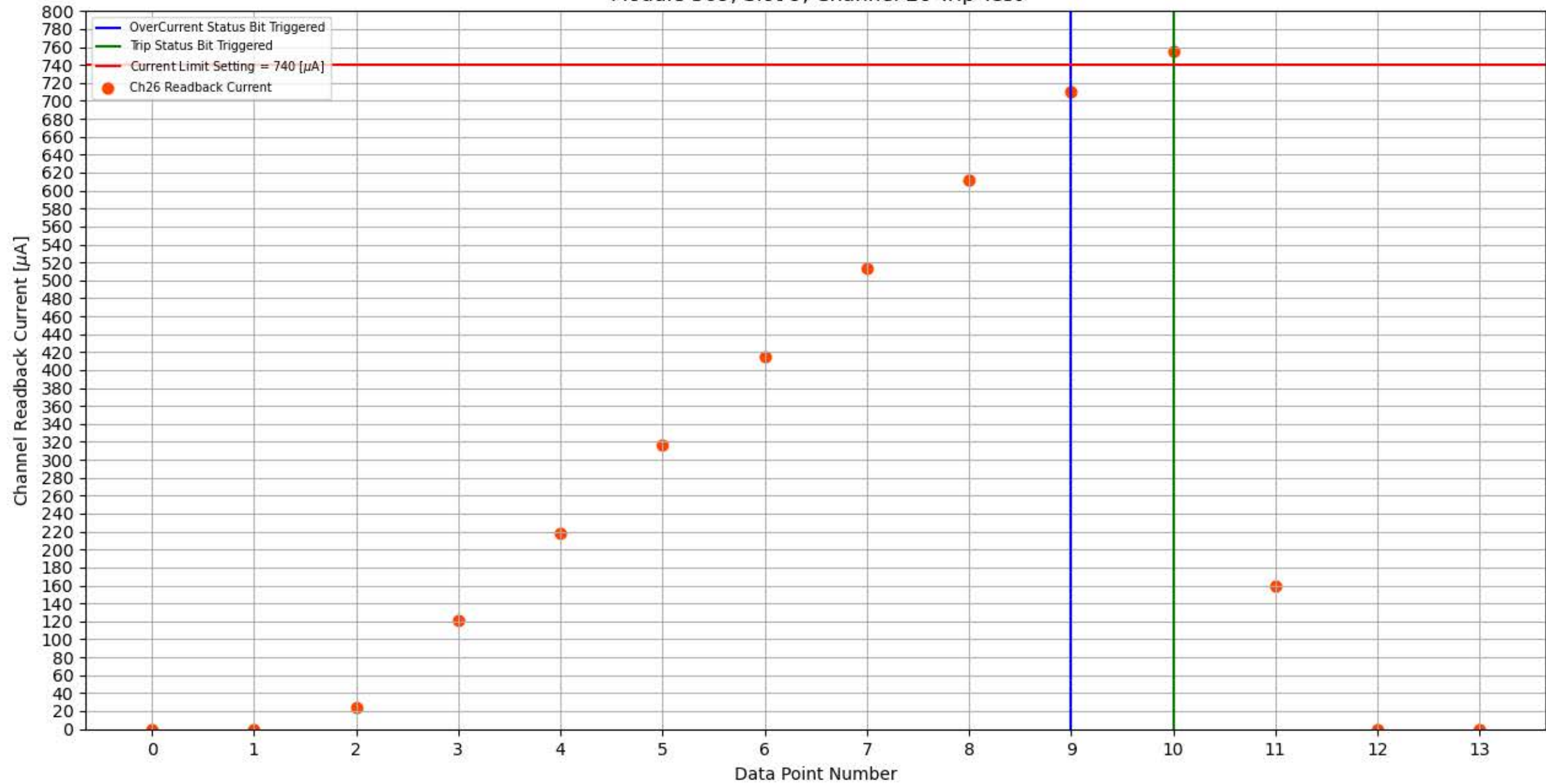
Module 309, Slot 9, Channel 26 Trip Test
