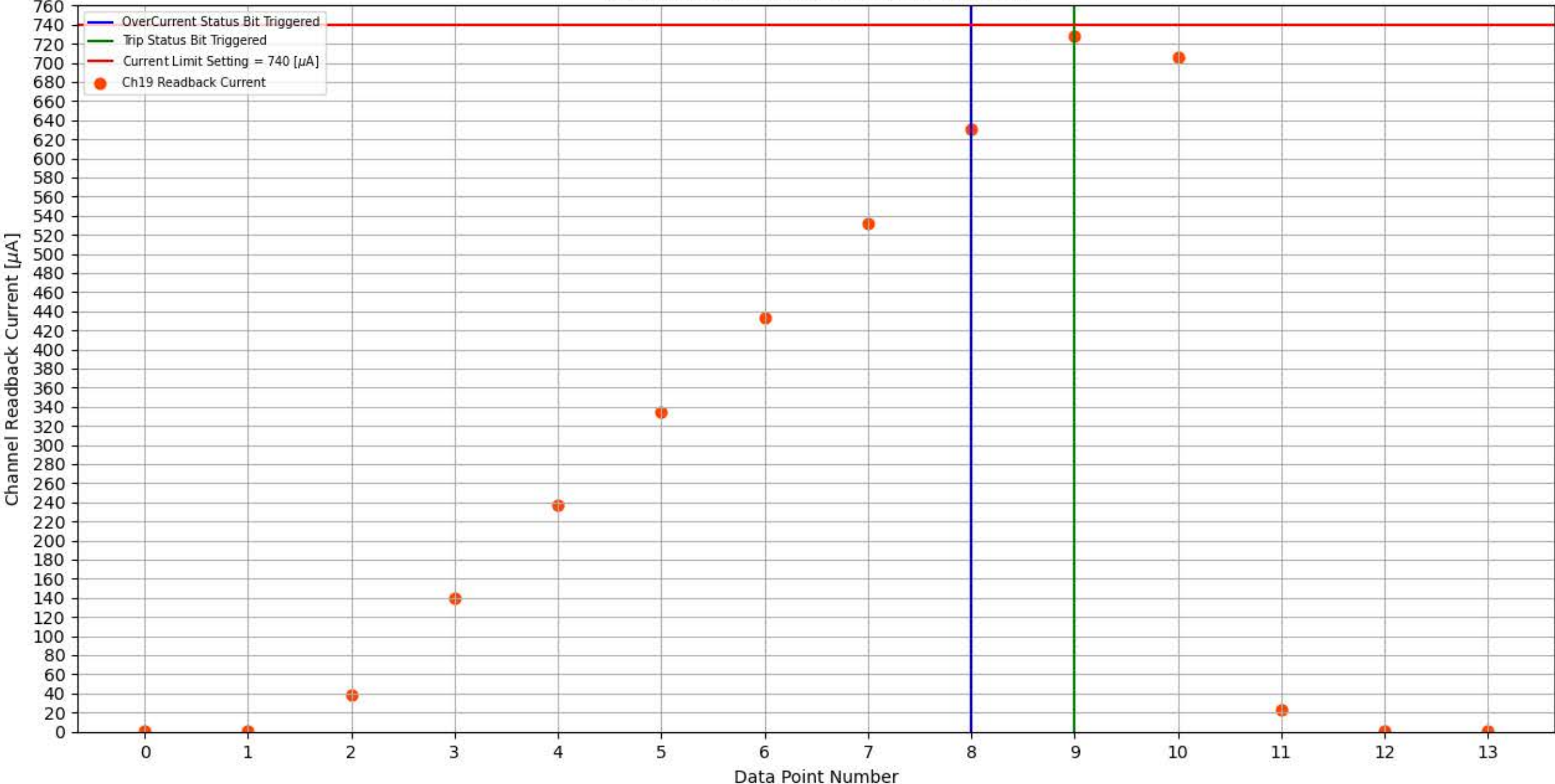
Module 309, Slot 9, Channel 19 Trip Test
