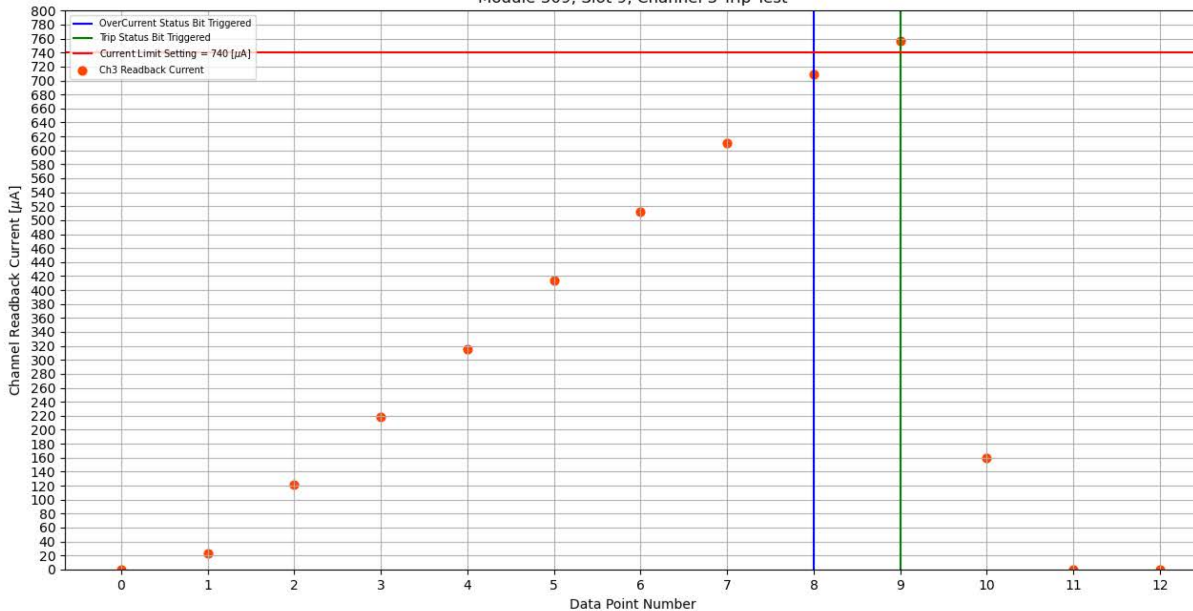
Module 309, Slot 9, Channel 3 Trip Test
