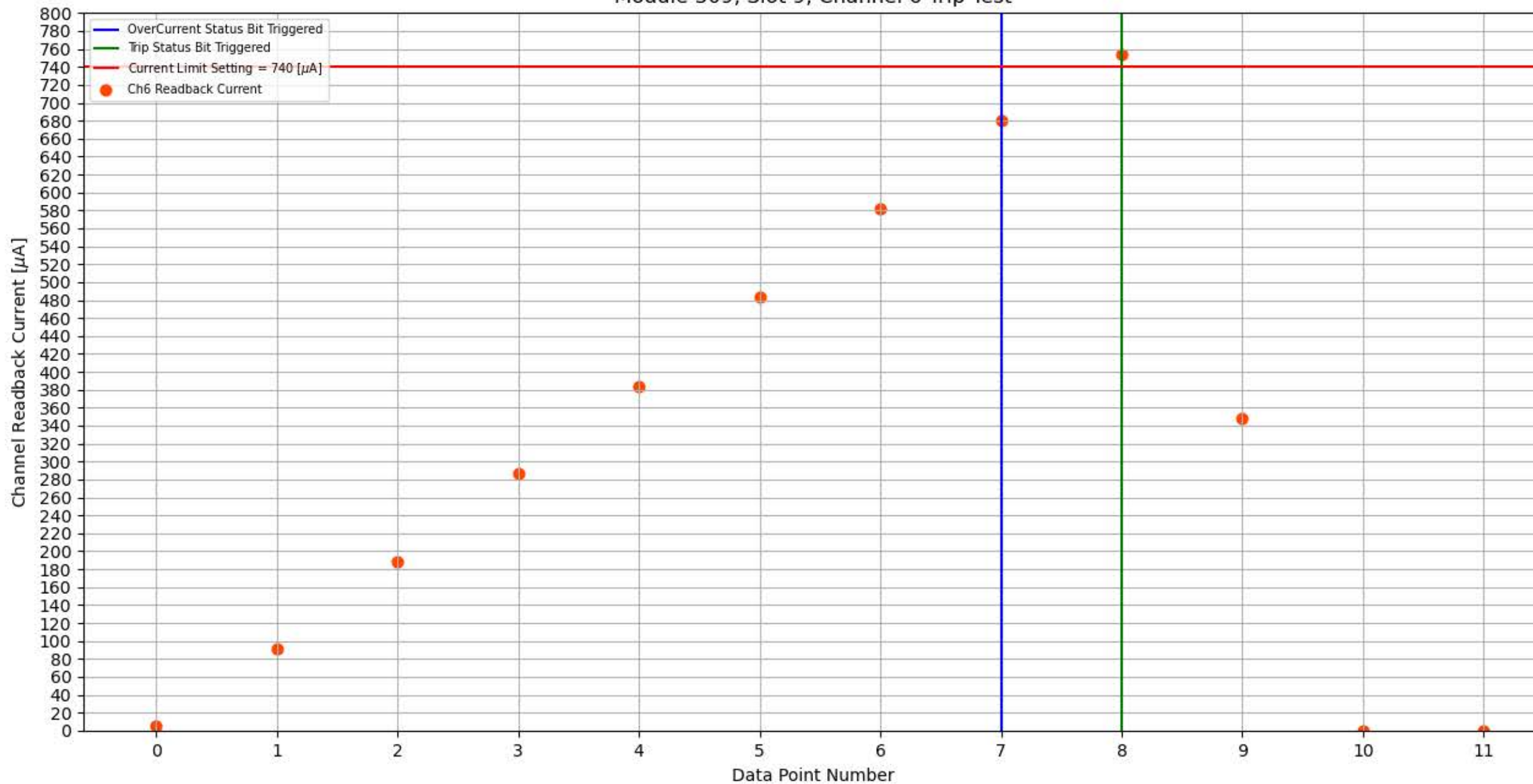
Module 309, Slot 9, Channel 6 Trip Test
