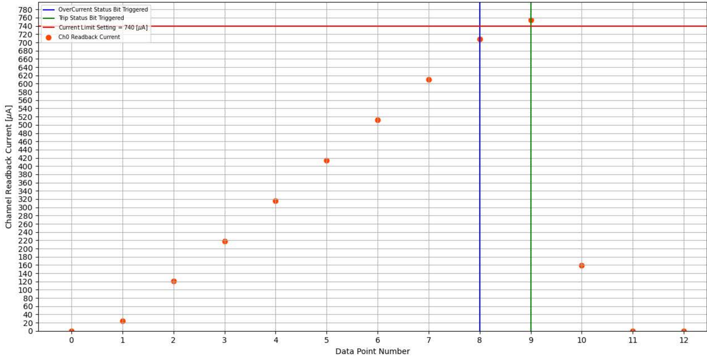
Module 309, Slot 9, Channel 0 Trip Test
