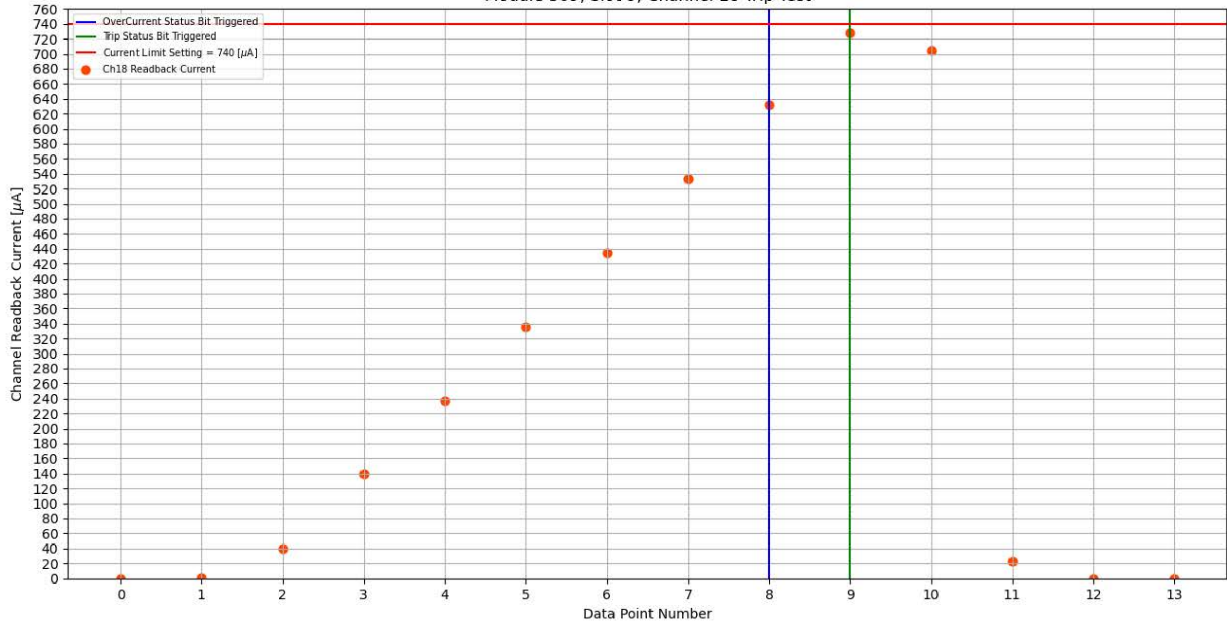
Module 309, Slot 9, Channel 18 Trip Test
