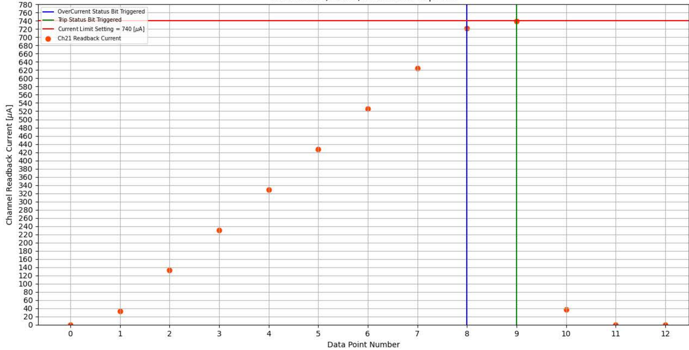
Module 309, Slot 9, Channel 21 Trip Test
