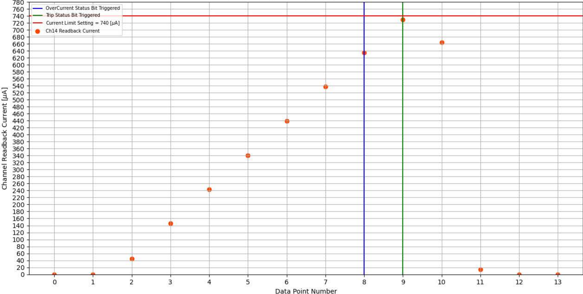
Module 309, Slot 9, Channel 14 Trip Test
