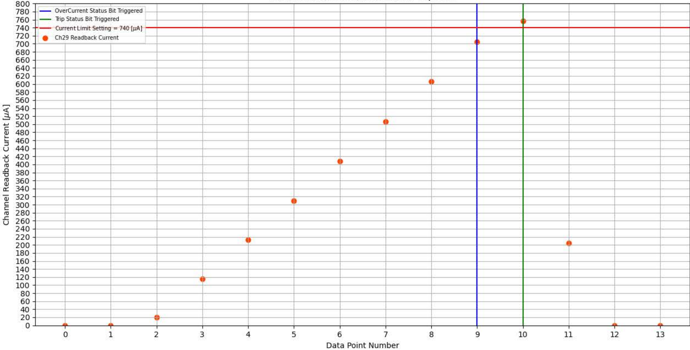
Module 309, Slot 9, Channel 29 Trip Test
