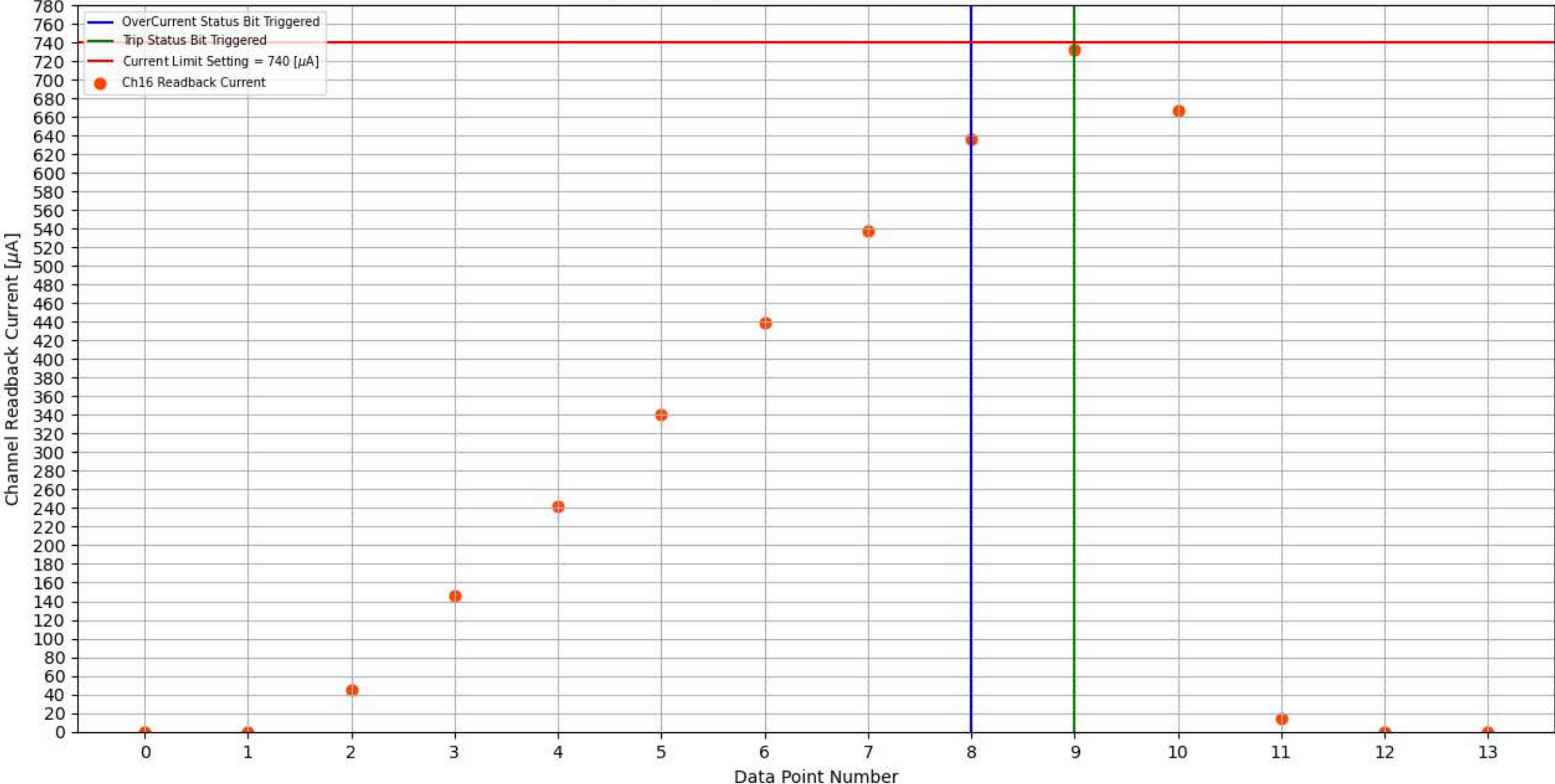
Module 309, Slot 9, Channel 16 Trip Test
