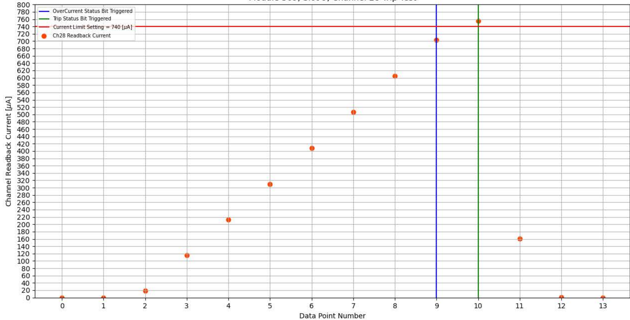
Module 309, Slot 9, Channel 28 Trip Test
