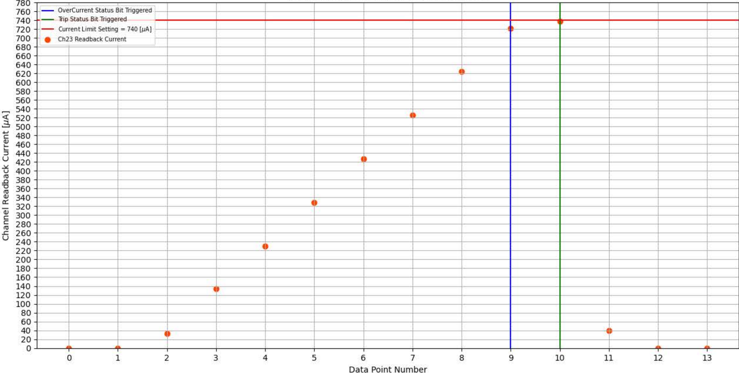
Module 309, Slot 9, Channel 23 Trip Test
