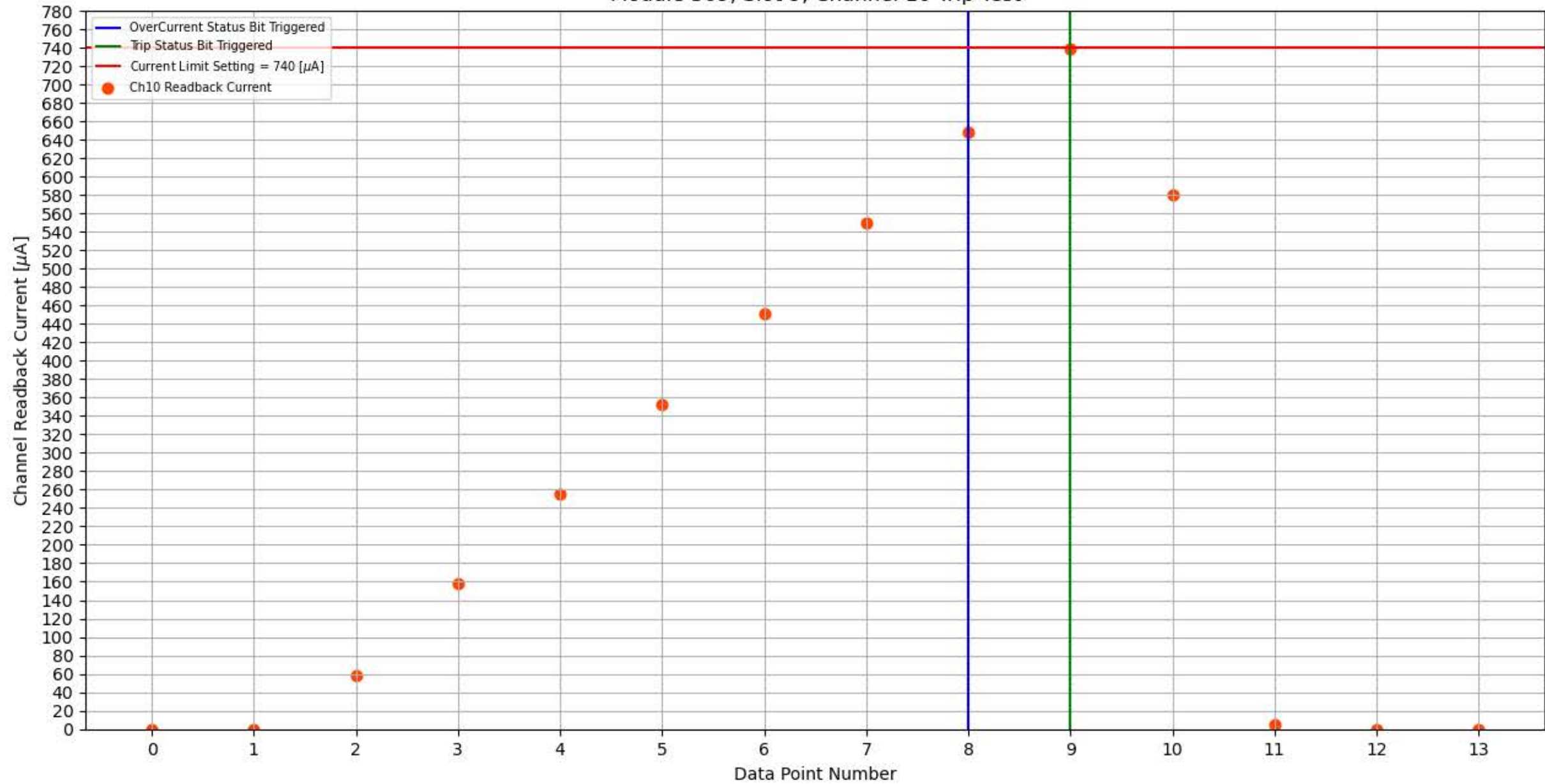
Module 309, Slot 9, Channel 10 Trip Test
