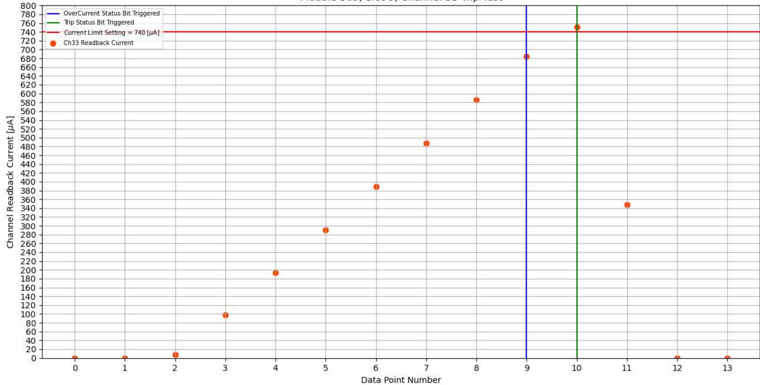
Module 309, Slot 9, Channel 33 Trip Test
