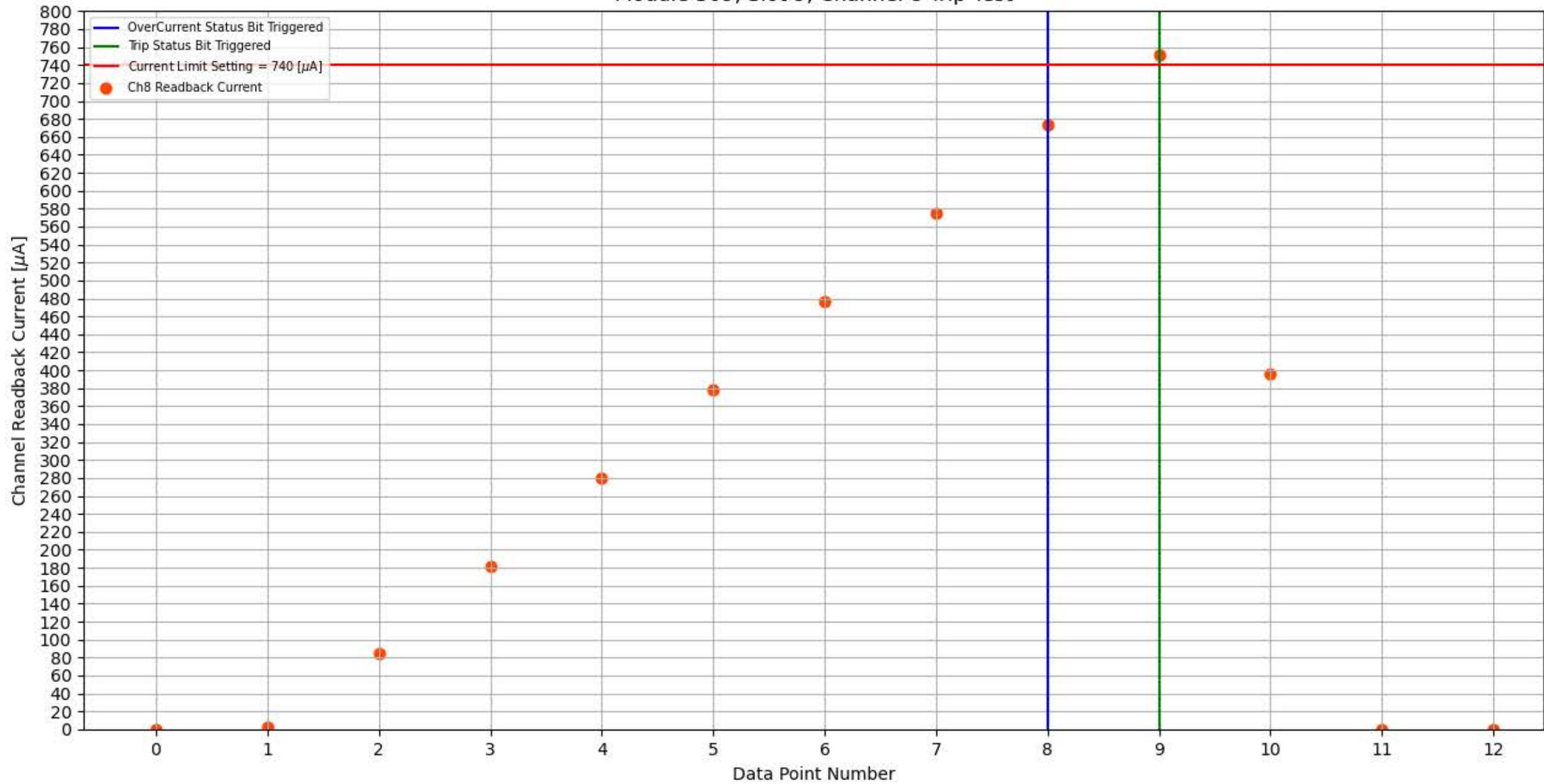
Module 309, Slot 9, Channel 8 Trip Test
