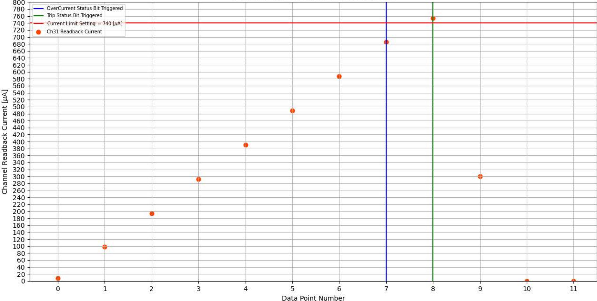
Module 309, Slot 9, Channel 31 Trip Test
