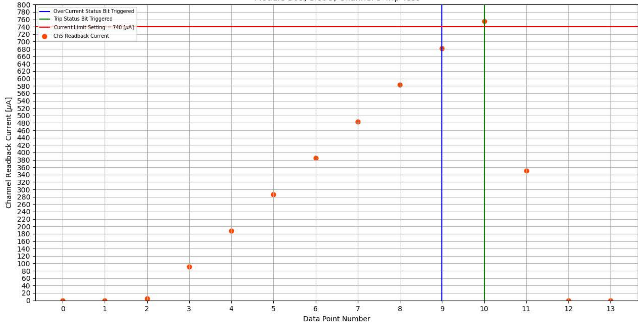
Module 309, Slot 9, Channel 5 Trip Test
