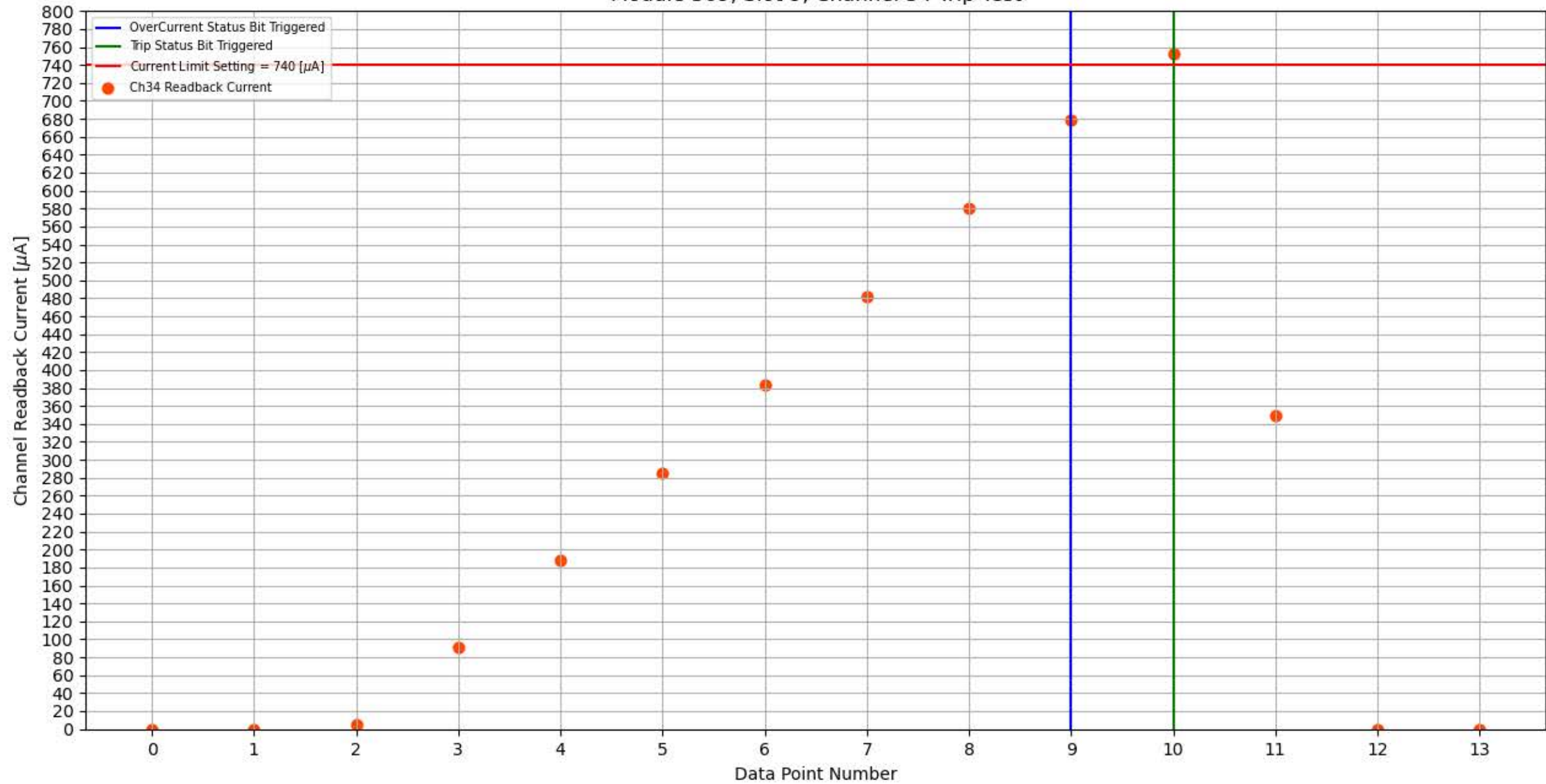
Module 309, Slot 9, Channel 34 Trip Test
