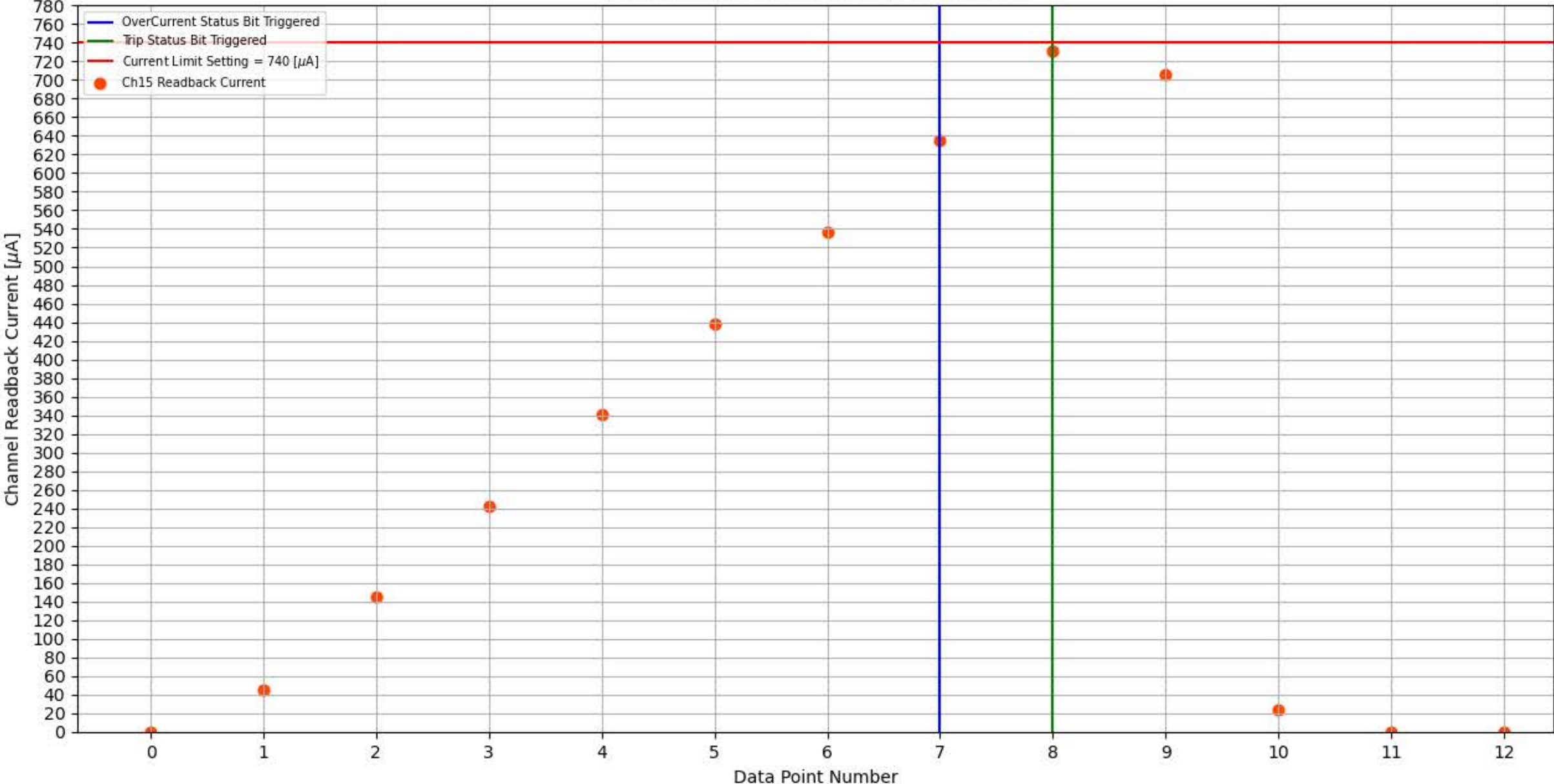
Module 309, Slot 9, Channel 15 Trip Test
