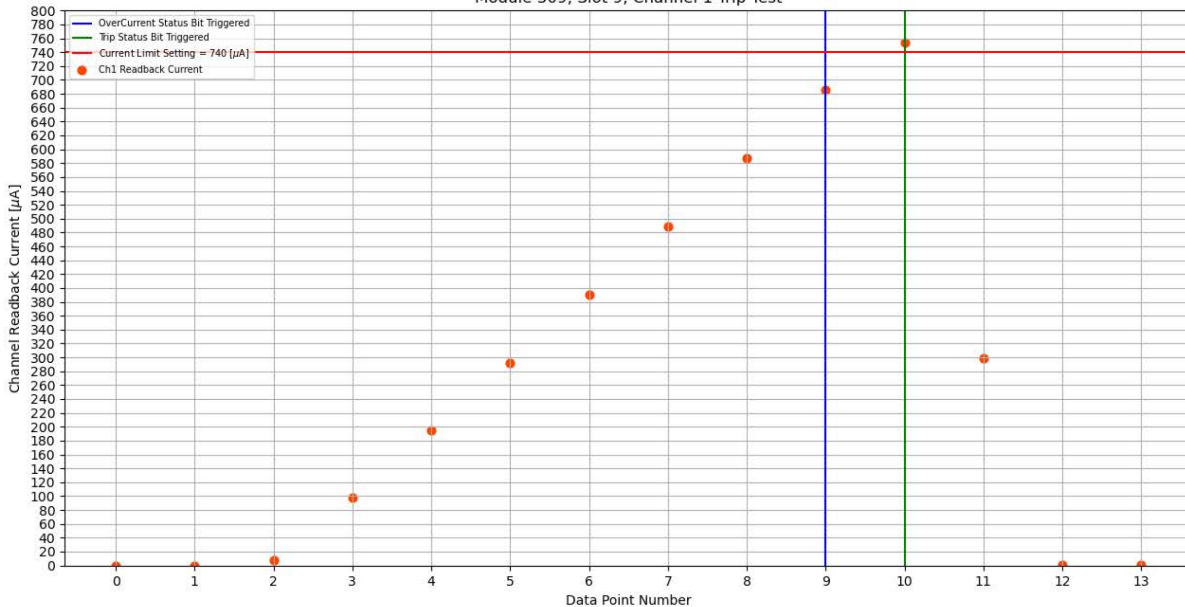
Module 309, Slot 9, Channel 1 Trip Test
