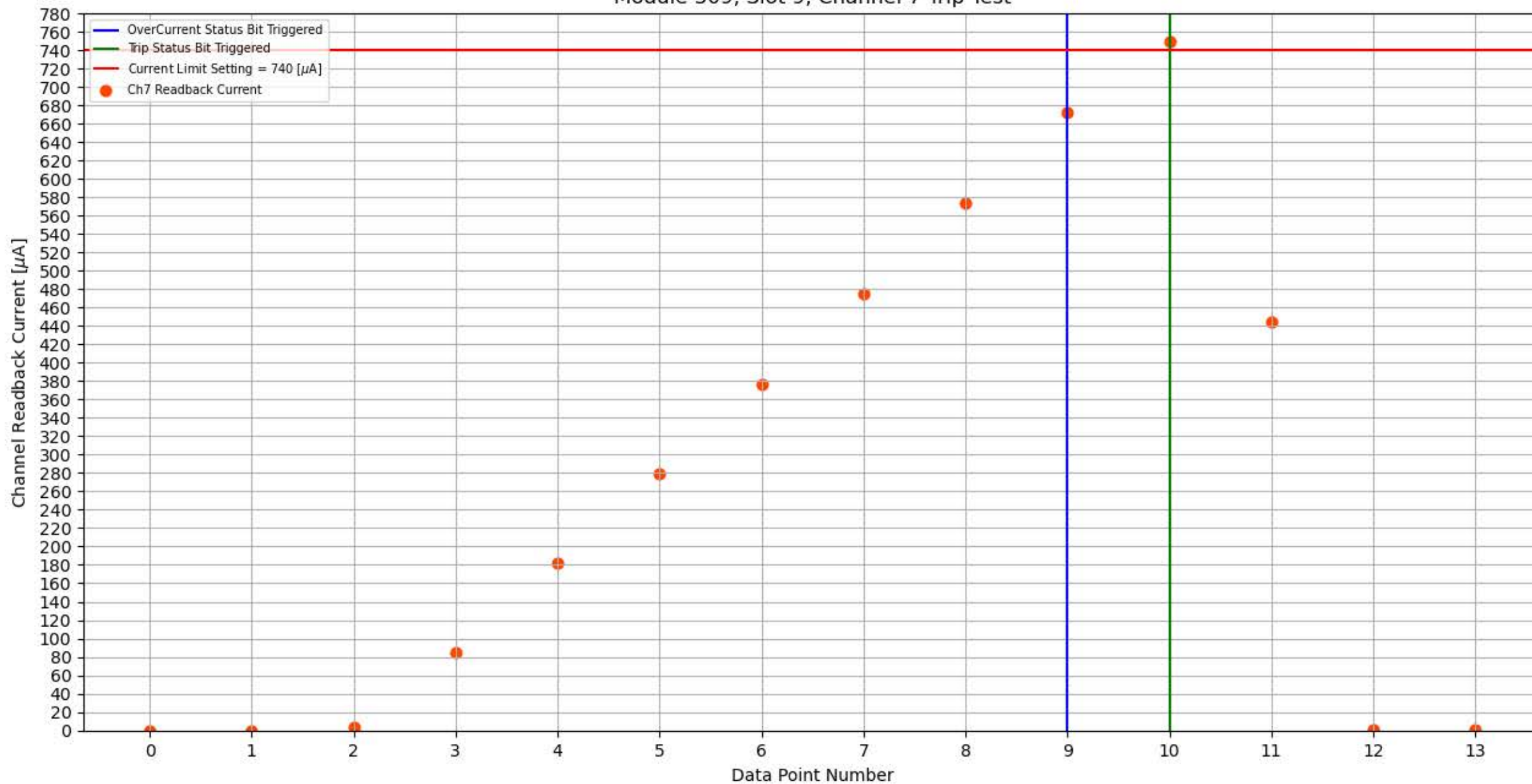
Module 309, Slot 9, Channel 7 Trip Test
