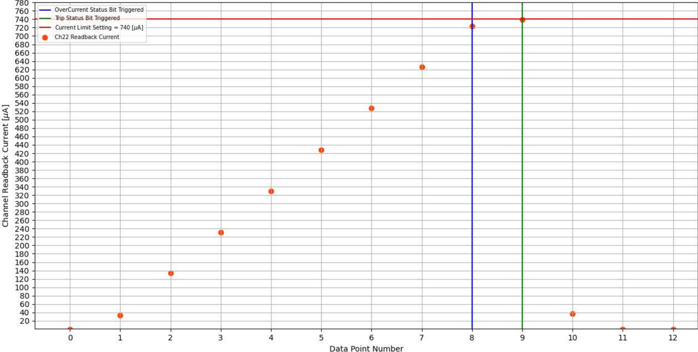
Module 309, Slot 9, Channel 22 Trip Test
