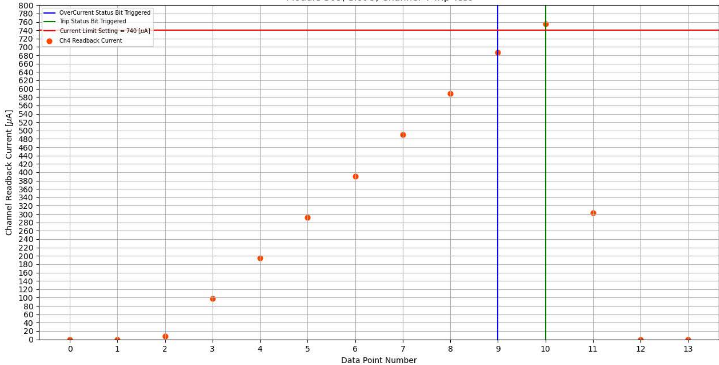
Module 309, Slot 9, Channel 4 Trip Test
