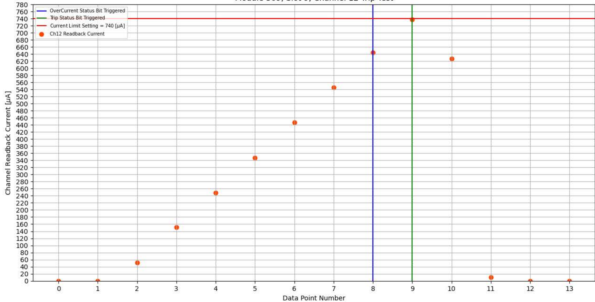
Module 309, Slot 9, Channel 12 Trip Test
