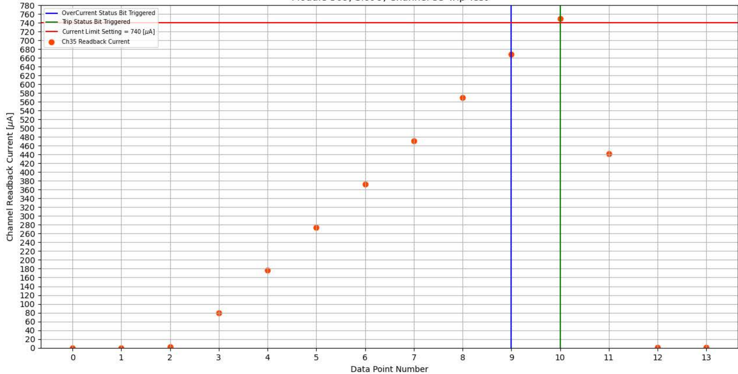
Module 309, Slot 9, Channel 35 Trip Test
