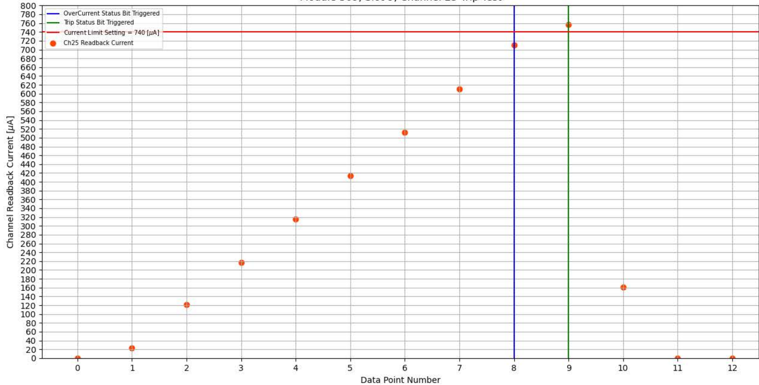
Module 309, Slot 9, Channel 25 Trip Test
