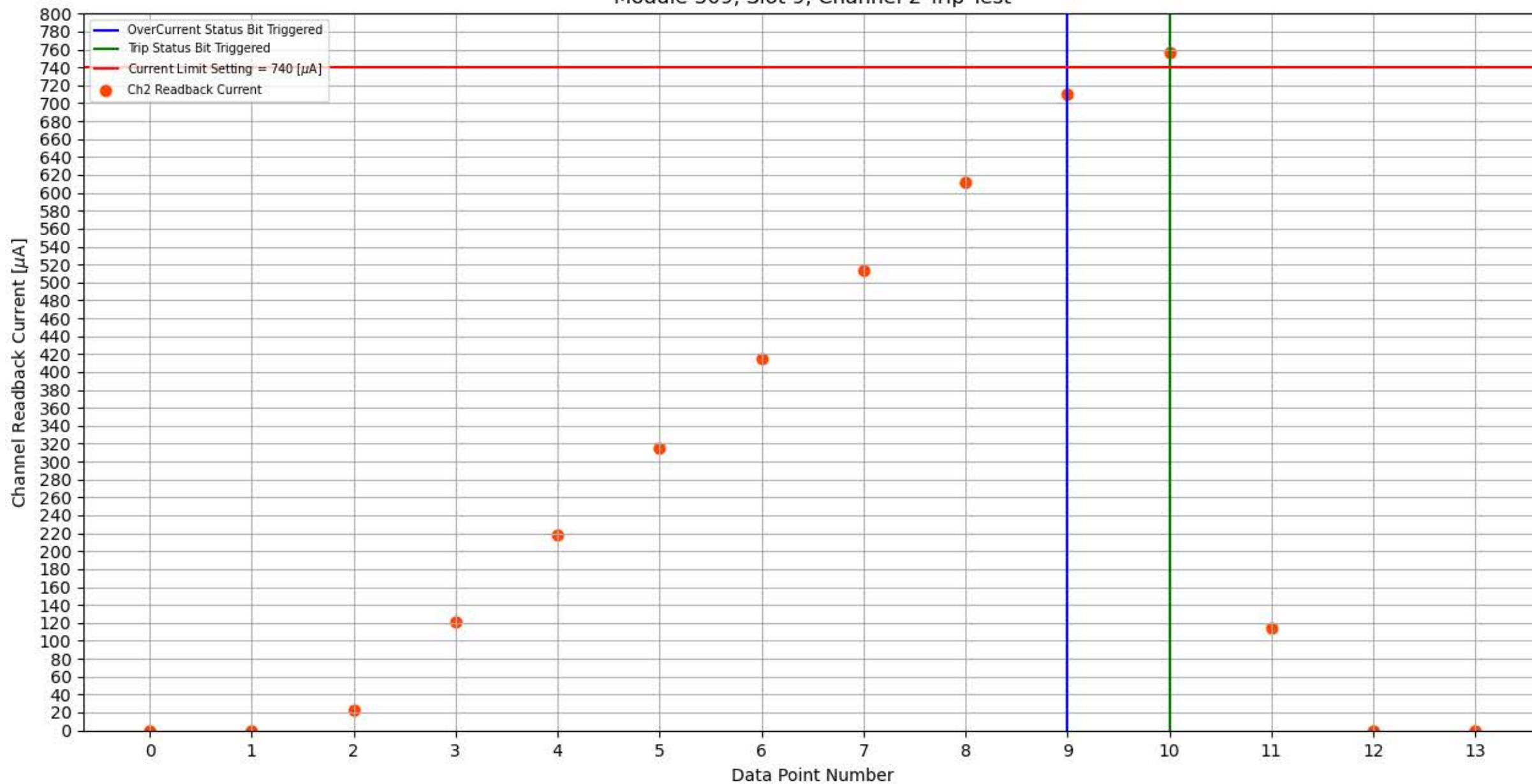
Module 309, Slot 9, Channel 2 Trip Test
