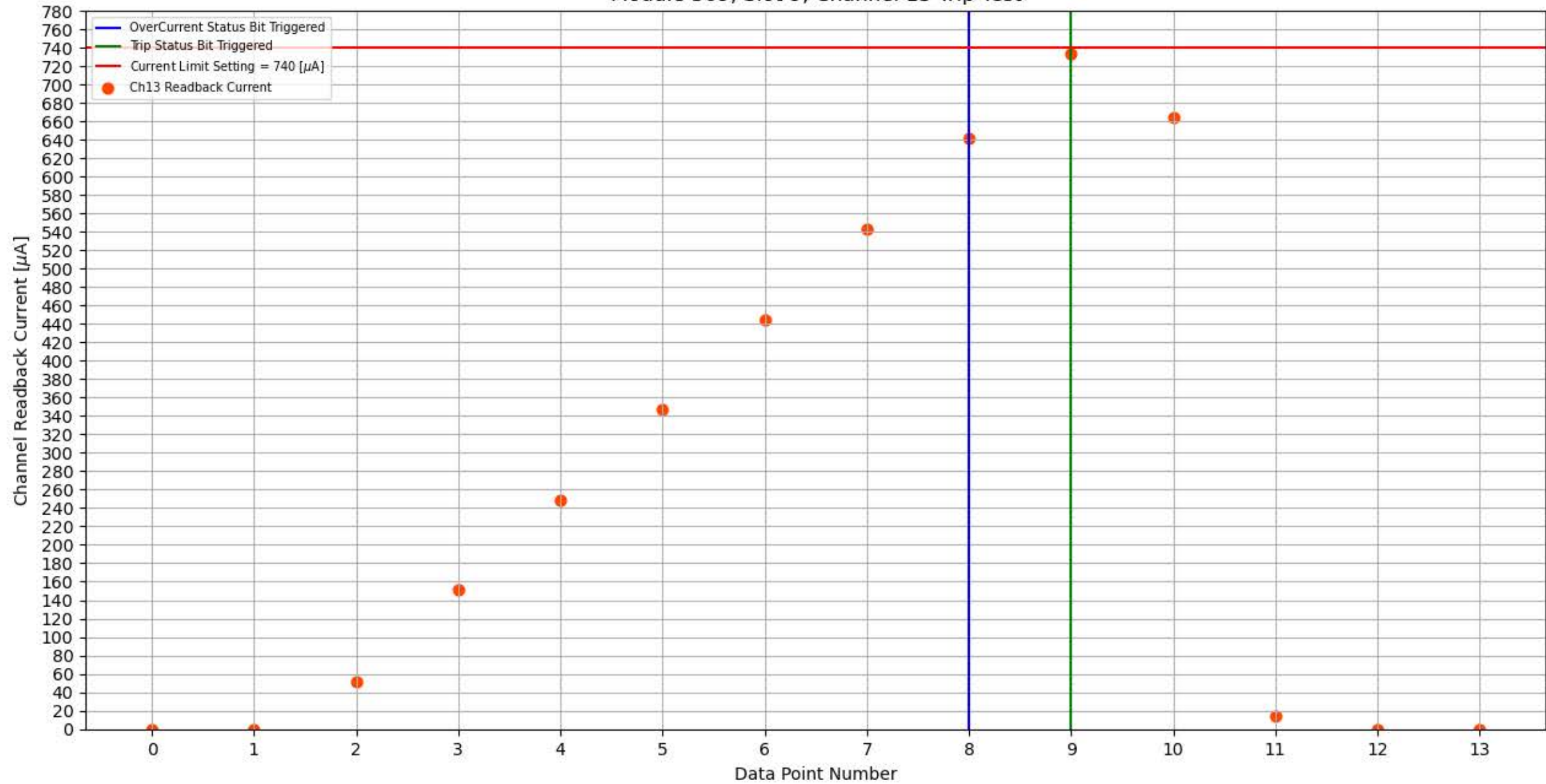
Module 309, Slot 9, Channel 13 Trip Test
